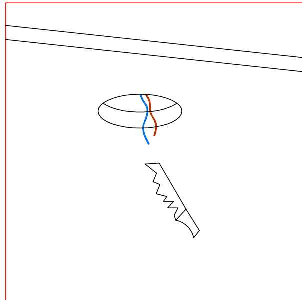
1. cut-out: Dia85mm.
