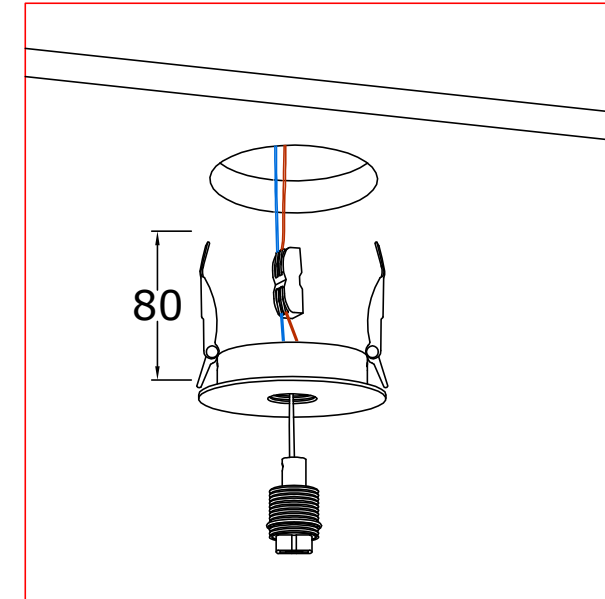
3. Both ends of the product spring buckle, vertical, put into the ceiling hole.
